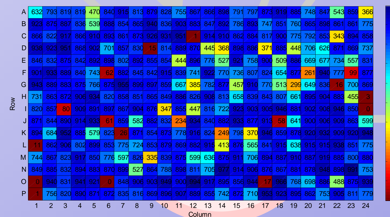
Figure 4: well quality values for a single plate
